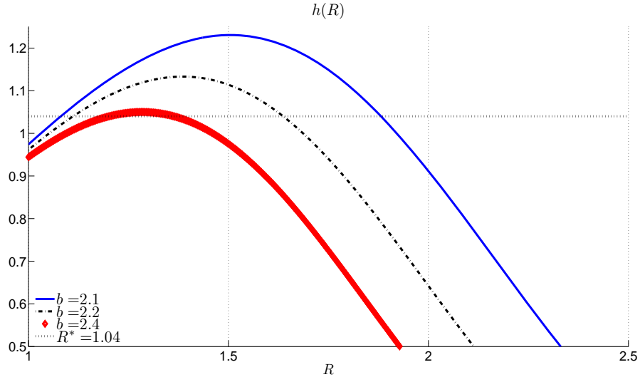
Figure 1: Expected return h(R; b)
