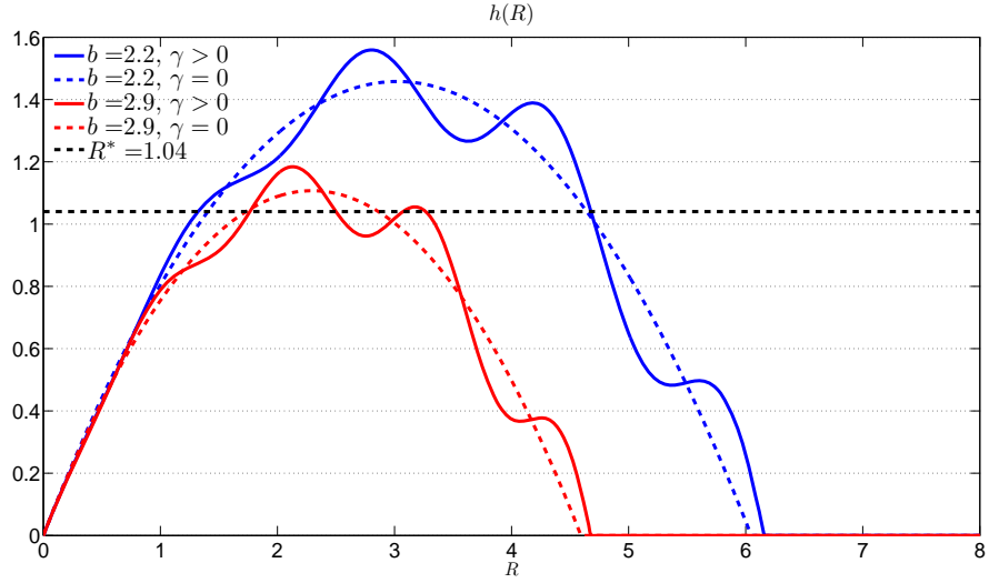
Figure 7: Perturbing the uniform distribution
