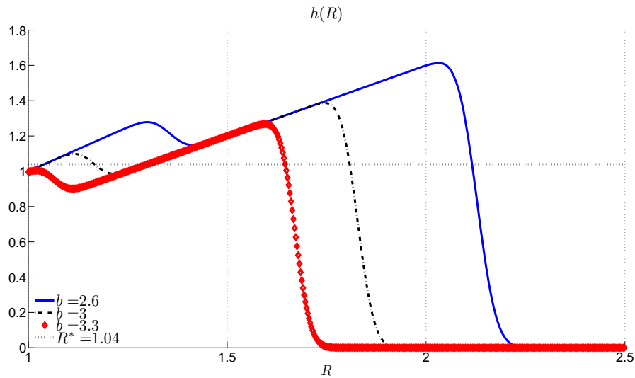
Figure 4: Expected return for the bimodal distribution
